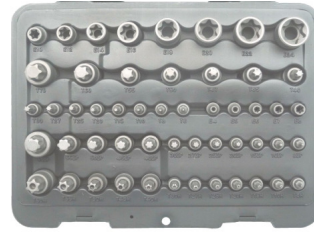
1165-WW Master set extra versterkte Torx ultra renforcé. T6 --> T70 / Torx Plus T8H-10H-15H-20H-25H-27H- 30H-40H-45H-50H-55H-60H / Tamper TX T8 --> T60IP / E4 --> E24 99 €
