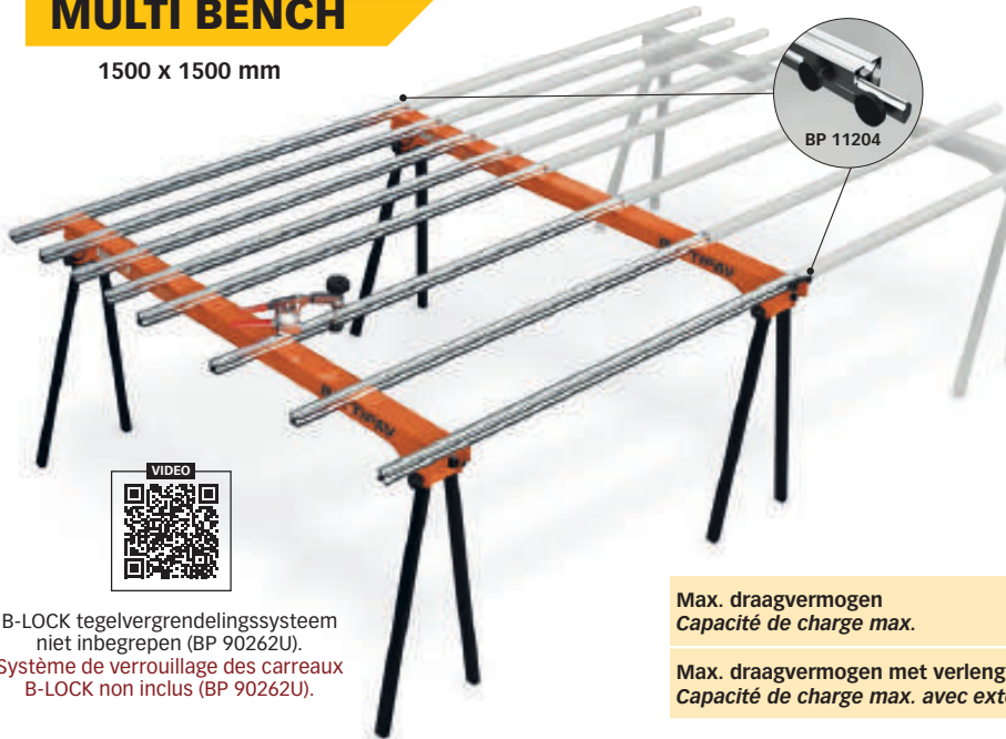
MULTI BENCH Ref. BP 11201
